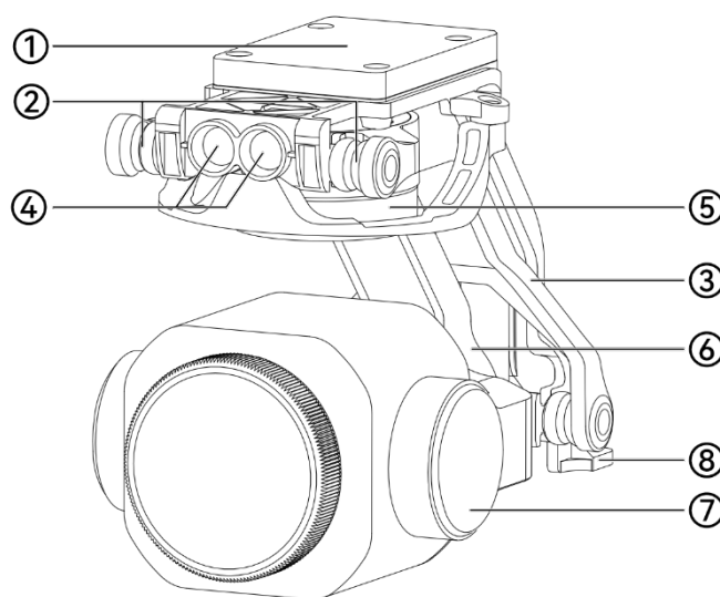
Fig 3-12 Gimbal Structure
